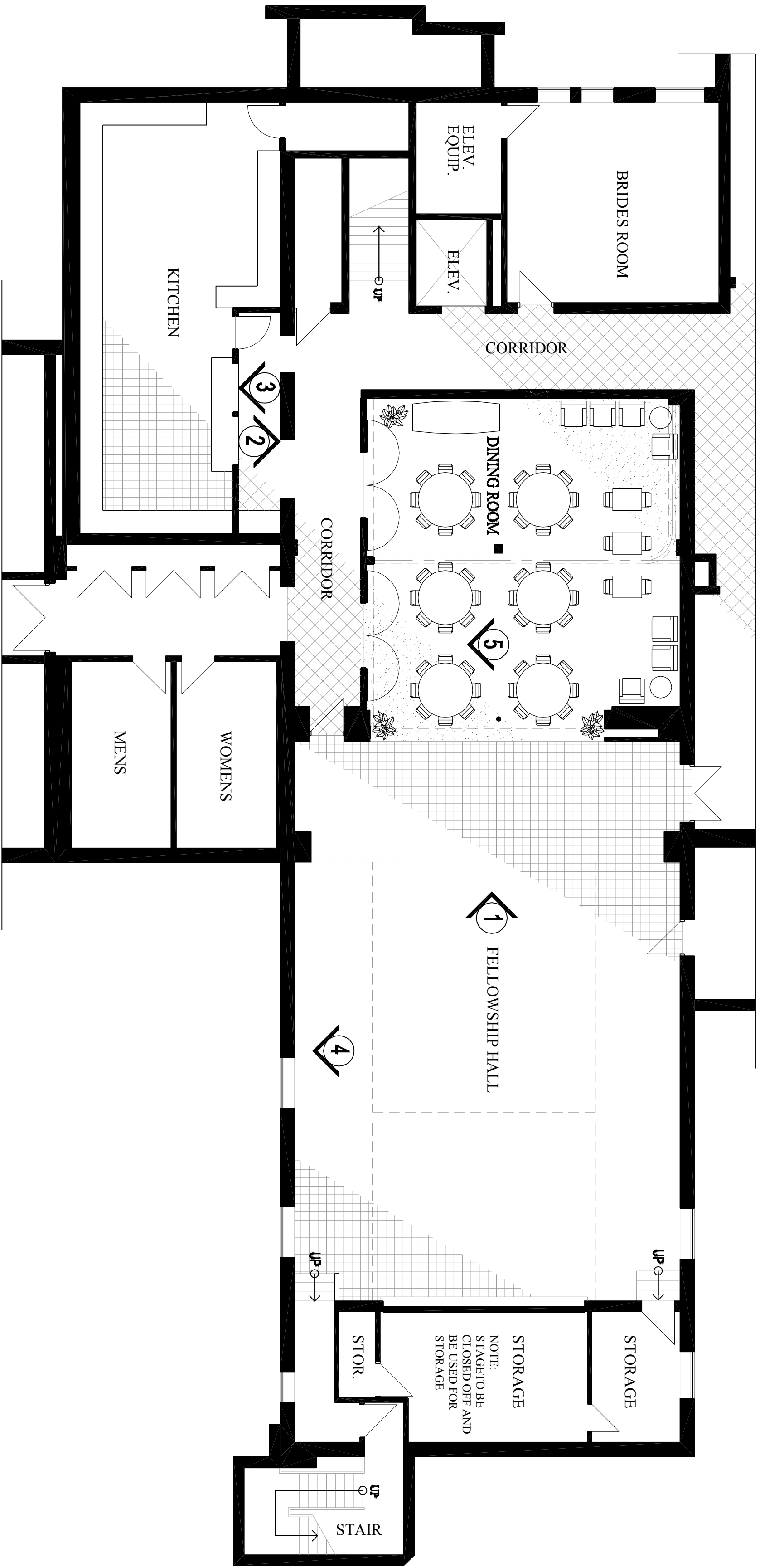
PROPOSED NICHOL-WALCH AREA PLAN SCALE: 1/8" = 1'-0"
